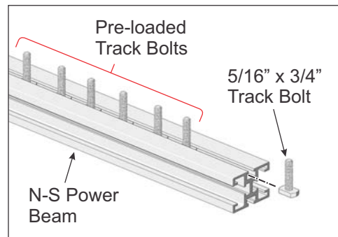
Figure 4-1: Pre-loading Track Bolts into N-S Power Beams
