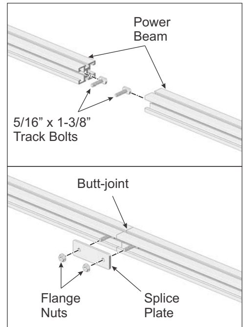
Figure 2-1: Splicing Power Beam with Splice Plate
