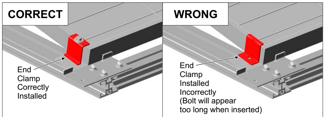
Figure 8-5: Correct and Wrong methods of installing Standard End Clamp
