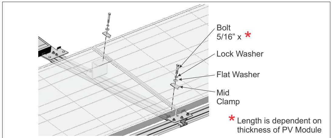
Figure 14-7: Installing Mid Clamps into Front and Rear Tilt Brackets
