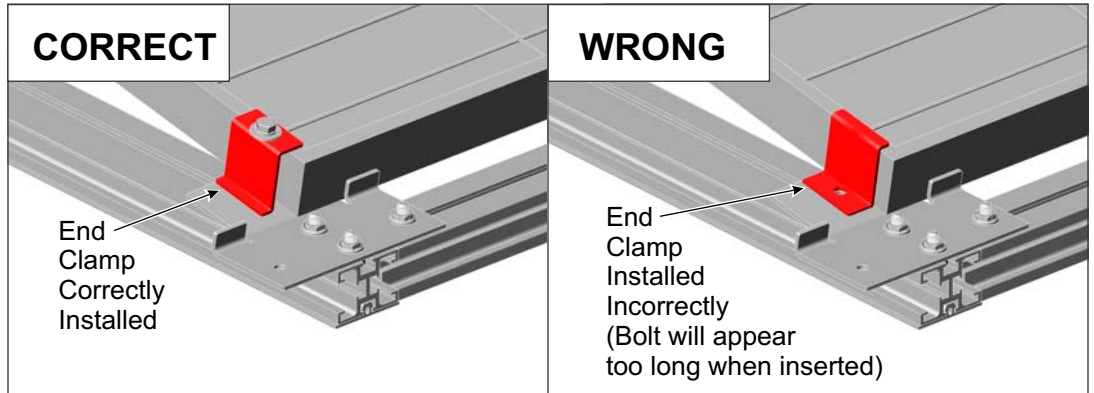
Figure 14-3: Correct and Wrong methods of installing Standard End-Clamp
