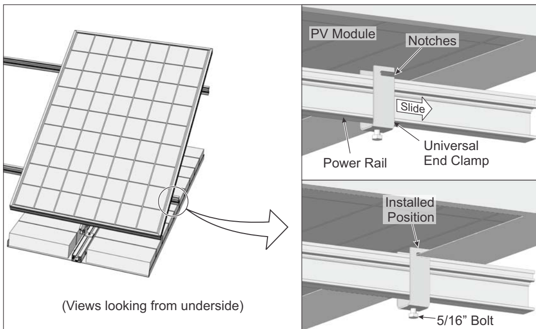
Figure 12-1: Installing PV Modules using Universal End Clamp
