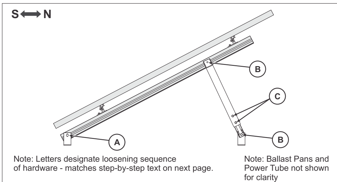
Figure 13-1: Adjusting Tilt Angle
