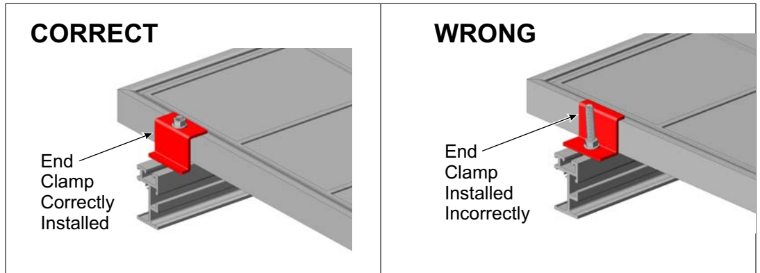
Figure 12-2: Correct and Wrong methods of installing Standard End Clamp
